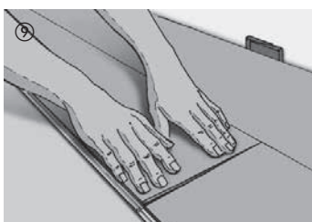
9 The board is then lowered in on the short side. Ensure here that the board is flush at the short side with the previously laid board. Pressure applied briefly to the side joint clicks in the board.
