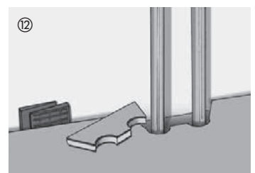
12 If radiator pipes protrude from the floor, drill or saw a cutout into the board (the size of the cutout depends on the radiator pipe and the required expansion space).
