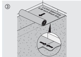
3 For sound insulation and to smooth out slight irregularities of the subfloor, unroll 1.4 mm thick Silent Grip underlay. Do not overlap. Our range of accessories also offers alternative insulation underlays. Asphalt-bitumen felt is not suitable for sound insulation.
