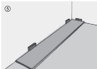
5 Starting in the right-hand corner of the room, align the boards of the first row with the tongue side parallel to the wall, and fix them in place with wall spacers as you proceed (always keep an expansion gap of 7-10 mm (3/8" - 1/2") around perimeter).
