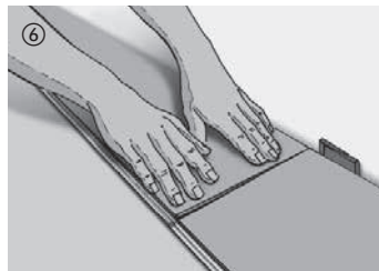
6 The remaining boards of the first row must be clicked in from above at the head ends into the previous boards. Pressure applied briefly to the side joint clicks in the board into the adjacent board. It is important to ensure that the first row is straight and exactly parallel to the wall. Cut the last board of the first row to size, leaving an expansion gap of 7 - 10 mm (9/32" - 13/32") between the board and wall. Fit in the board and lay it flat.
